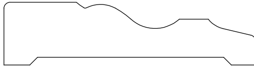
CASING 125023 5/8" X 2 1/2"
