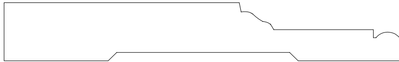
CASING 142533 5/8 X 4 1/4"
