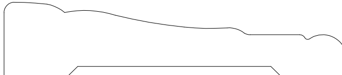
CASING 132510 11/16" X 3 1/4" (SIMILAR TO MDF 445M)
